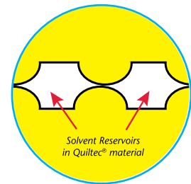
Cross-section of Quiltec® 2-ply material
